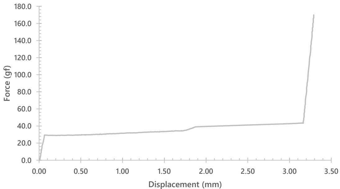
Kailh Box Spring (Image) (Upstroke)
